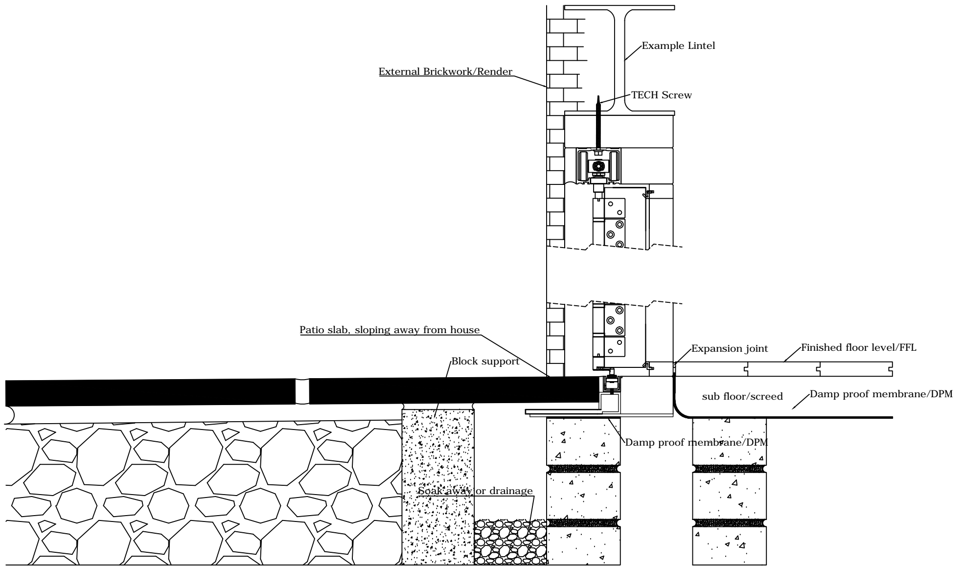
Valdi Ltd - Top Hung Folding Sliding Doors - Flush Patio Sill - Raised Patio Construction
